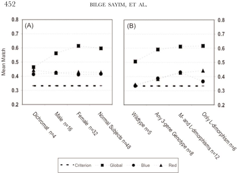
Figure 9. Mean Matches Proportions for Subject Groups
